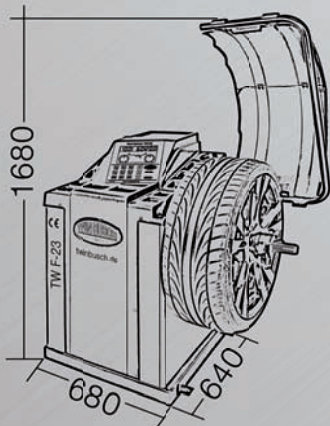
(1) 15 storage compartments (2) Accurate targeted mounting of all the weights using the electronic caliper arm (3) Integrated distance measurement (4) Quick release nut \varnothing = 40 mm (5) Digital Display (The new, compartment design ensures maximum user comfort and optimal ergonomics)
